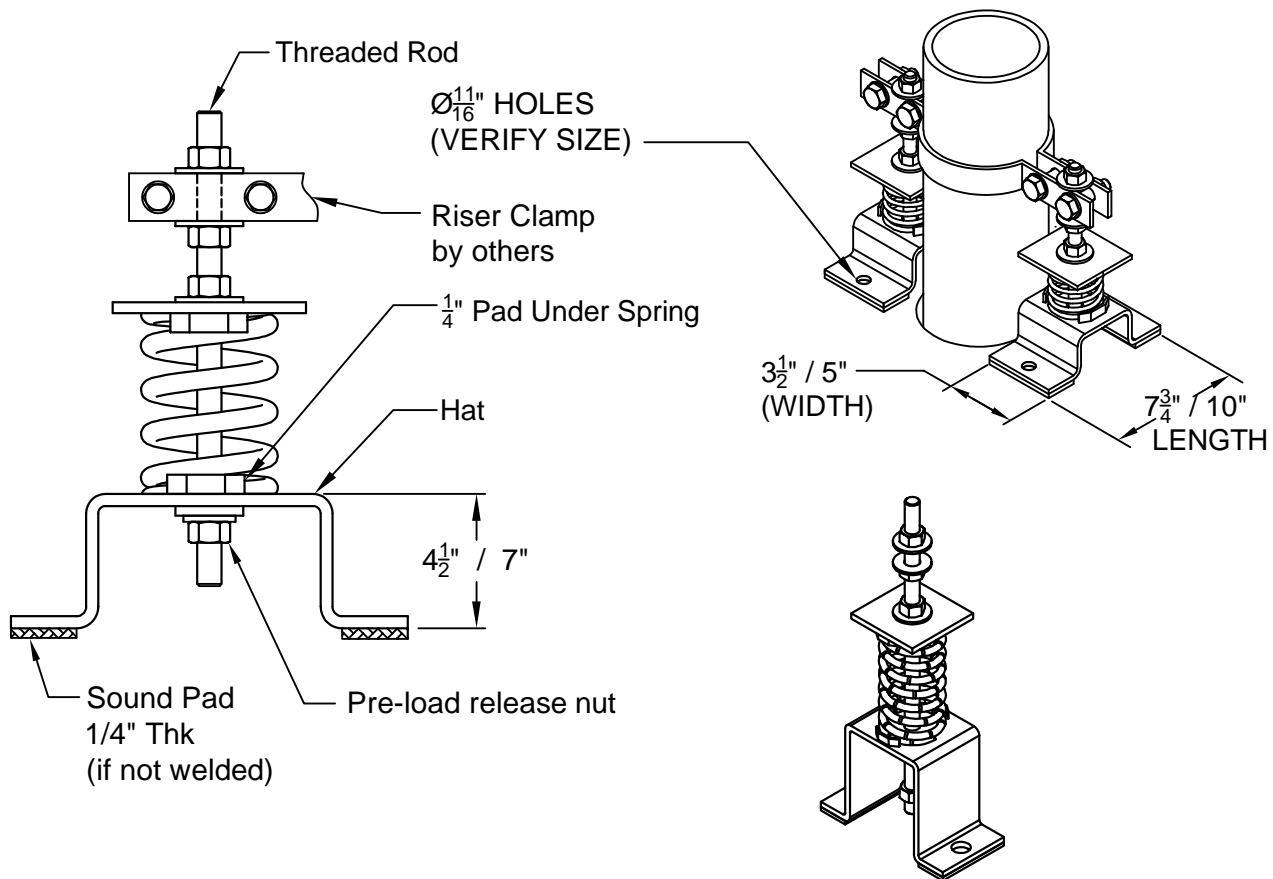
ISOMETRIC VIEW
