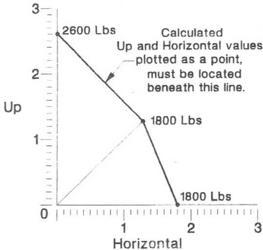
INTERACTION CURVE
